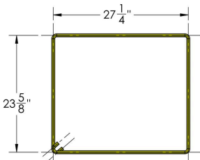
TYPE 1 #5 CLOSED TIE (VERTICAL)
