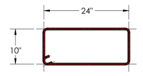
TYPE 2 #5 CLOSED TIE (HORIZONTAL)
