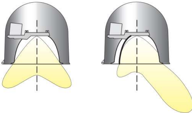
ASYMMETRIC EMISSION OBTAINED WITH ASYMMETRIC REFLECTOR ACCESS
