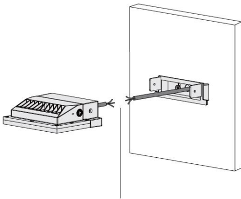
Connect the power cable
