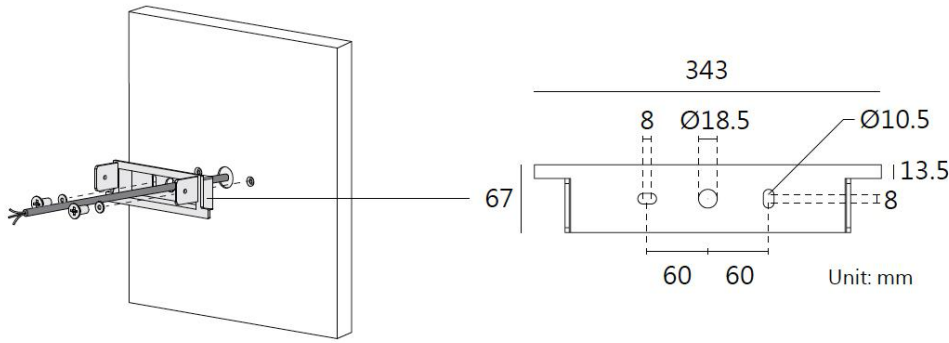
Secure the wall bracket
